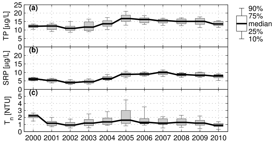
Figure 11: Annual concentrations measured in the LSC effluent for the 2000 - 2010 interval: (a) total phosphorus, (b) soluble reactive phosphorus, and (c) turbidity.
