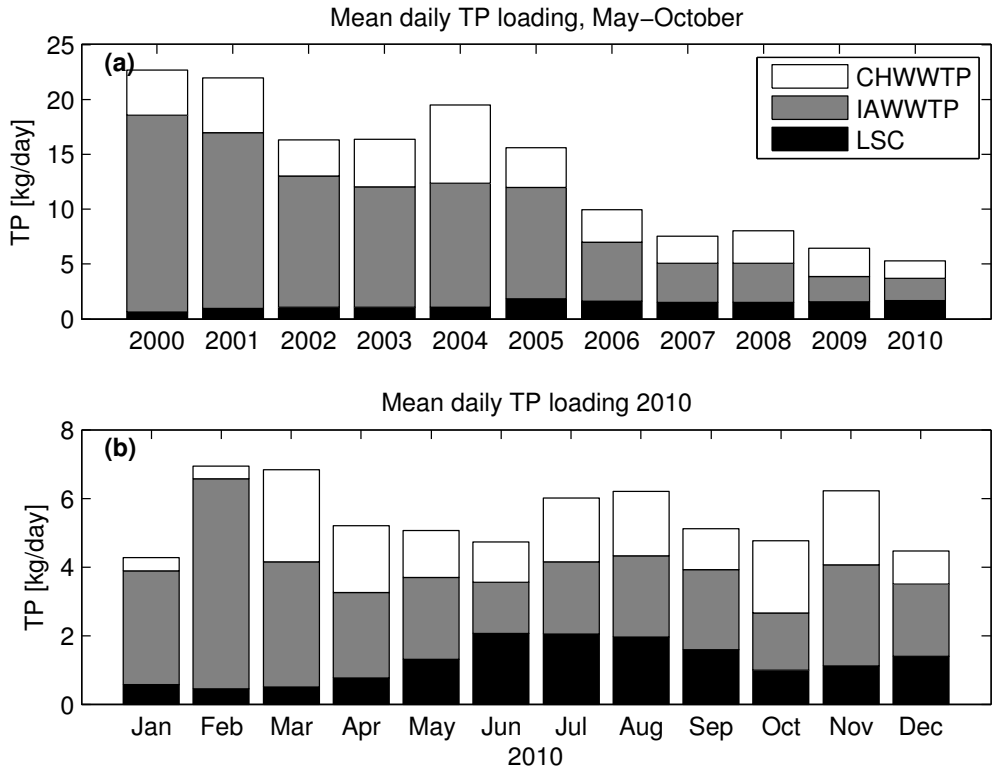
Figure 9: Trends in point source TP loading to the southern shelf: (a) mean daily loading in the May - October period, 2000 - 2010, (b) monthly mean loading in 2010.
