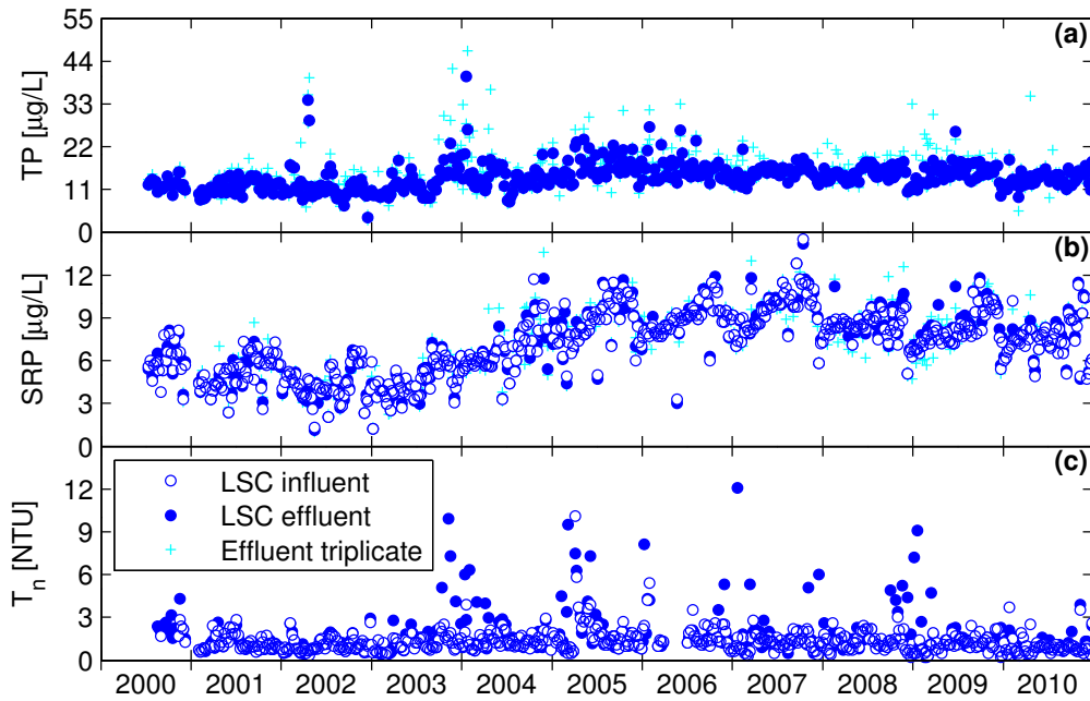
Figure 10: Time series of concentrations measured weekly in the LSC effluent for the 2000 - 2010 interval: (a) total phosphorus, (b) soluble reactive phosphorus, and (c) turbidity. The median of triplicate samples was used as the representative value. “+” symbols represent additional triplicate sample values.
