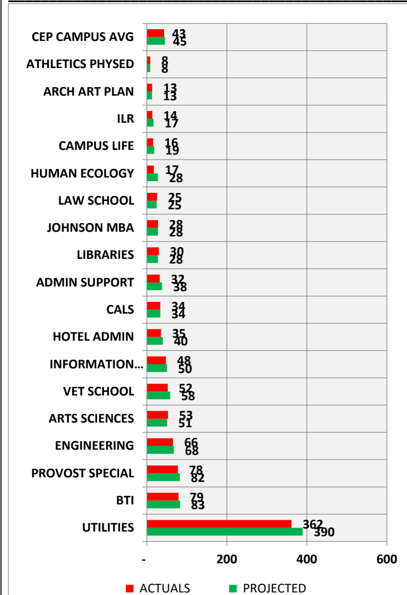
CHILLED WATER EUI (kBtu/gsf): 11.0 million GSF
